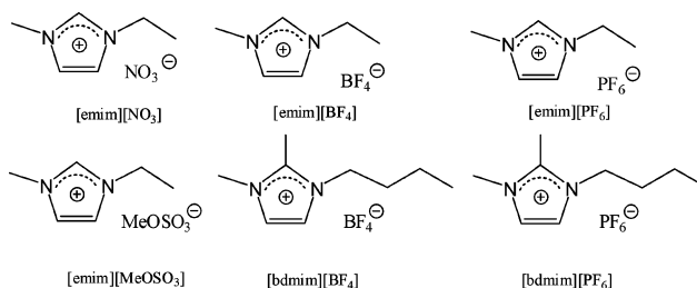
Scheme 1 Ionic liquids tested as additives.
